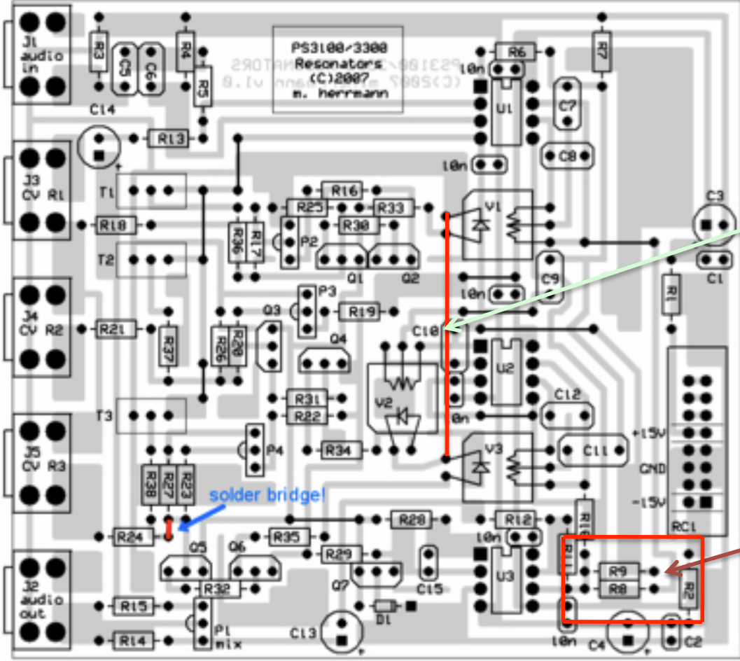
components diagram
